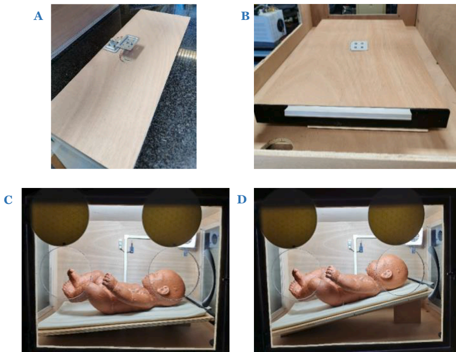
Fig. 3. (A) Weight sensor placement. (B) PLA structure with the handle. Inclination of the bed 6° (C) and 12° (D) by using the wooden wedges.
